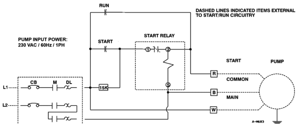
PUMP START/RUN CIRCUITRY DIAGRAM
